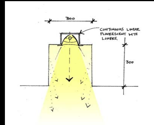
Recessed continuous 1x35W T-5 linear fluorescent luminaire with reflector and louver
