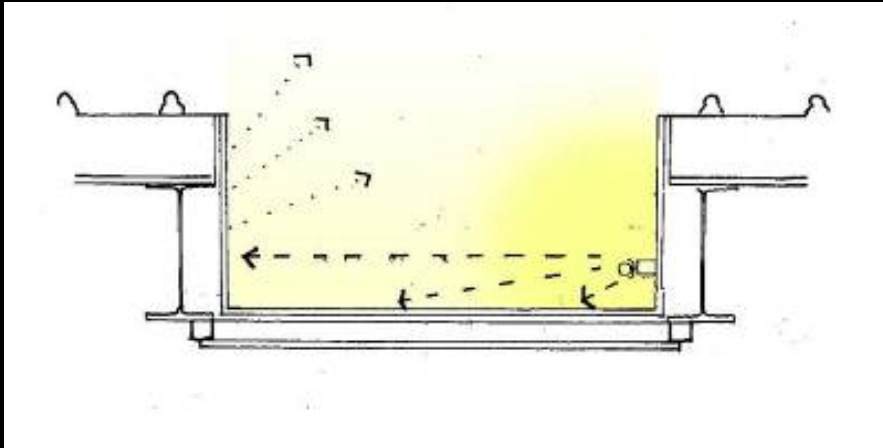
Interior of gutter lit with cold cathode
