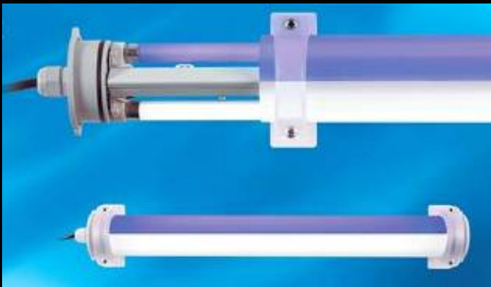
ENCAPSULITE 360 2X35W T-5 LINEAR FLUORESCENT WITH COLOURED UPLIGHT
